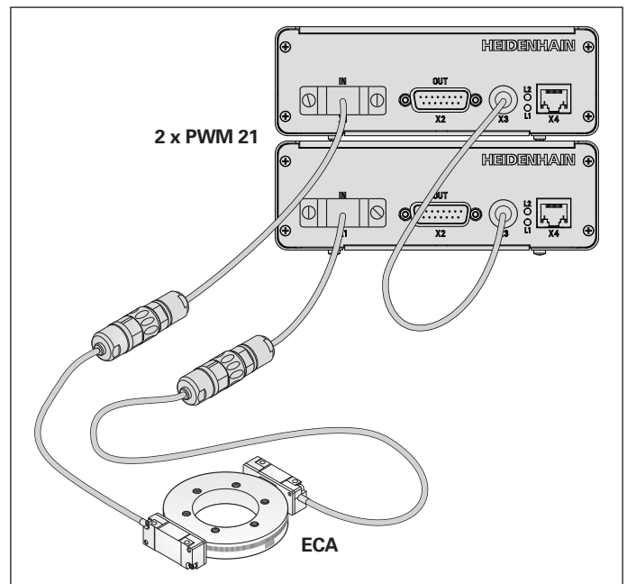
Compensation via a virtual reference with the PWM 21
