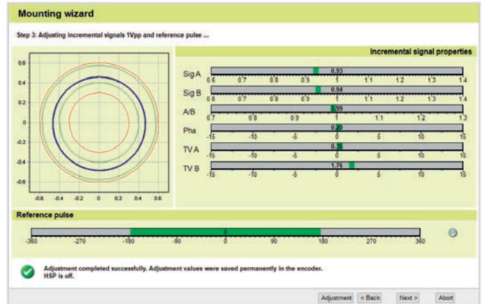
Mounting support for the ERA 4000 with the ATS software and PWM 21
