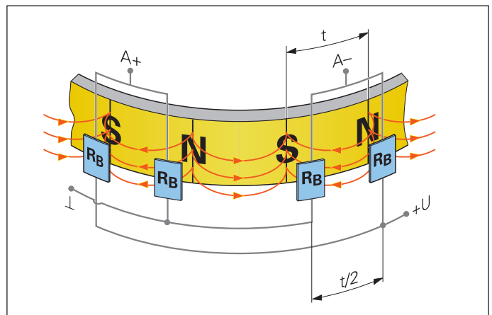
Magnetostrictive scanning principle
