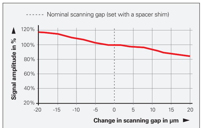
Influence of the scanning gap on the signal amplitude for the ERA 4000
