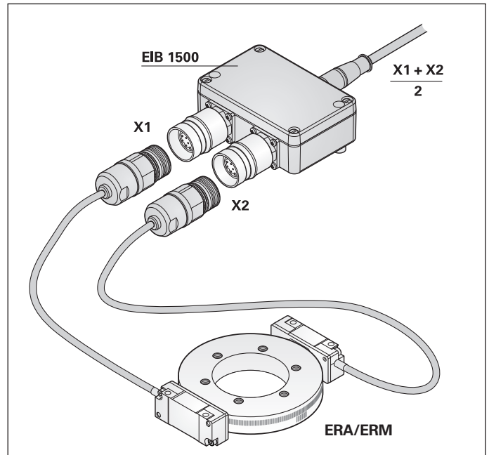
Compensation via position calculation (e.g., the EIB 1500)
