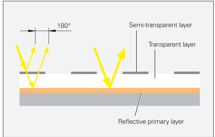
Design of a METALLUR graduation
