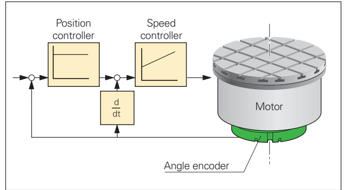
The position feedback from the angle encoder is used as the input for the position controller and speed controller
