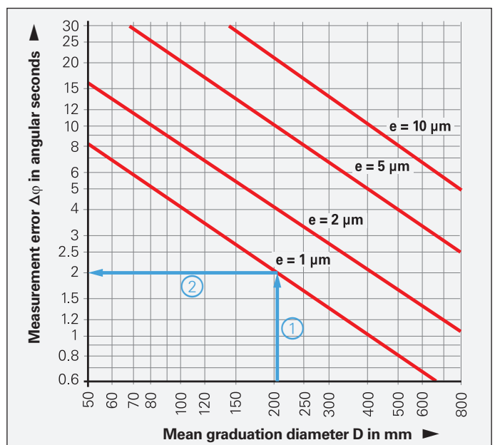
Resulting measurement error \Delta\varphi for various eccentricities e as a function of the mean graduation diameter D (with graph-reading example)
