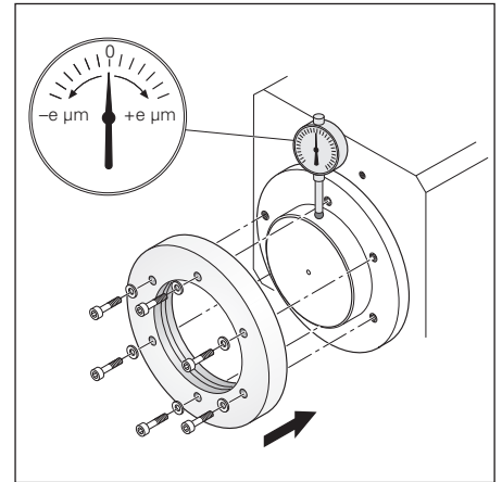
Centering via a centering collar
