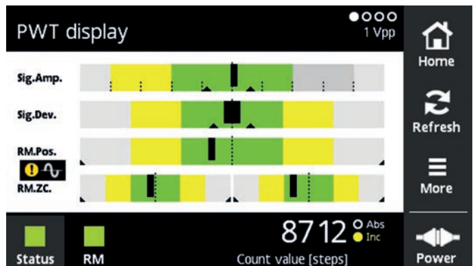
Functionality check, such as for the ERM 2000 with the PWT 101
