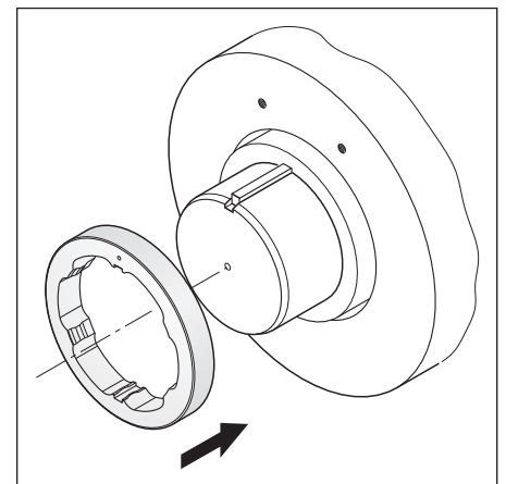
Mounting the scale drum TTR ERM 2405
