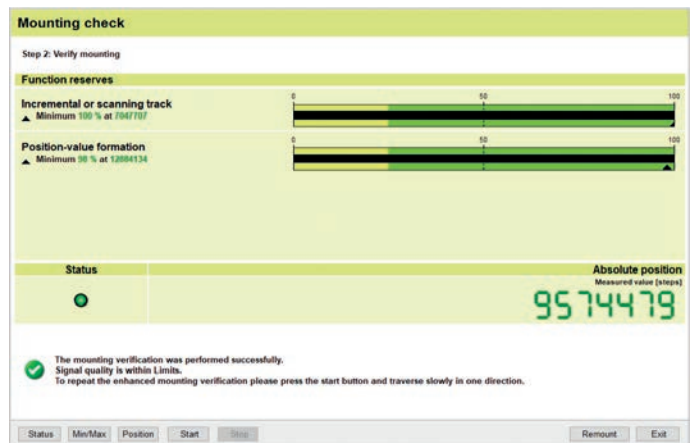
Mounting support, such as for the ECM 2000 with the PWM 21 and ATS software
