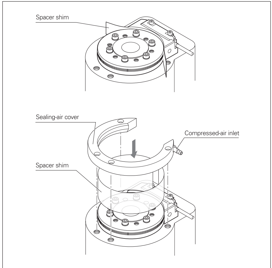
Mounting an ERA 4480 with sealing-air cover
