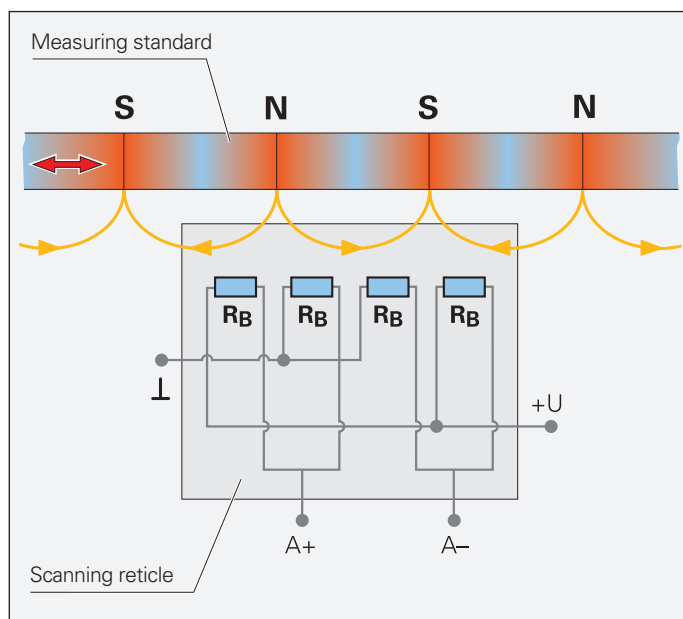
Magnetoresistive scanning principle
