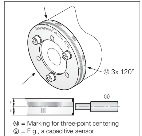
Three-point centering for the ERA
