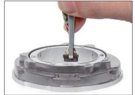
Mounting aid for output cable
